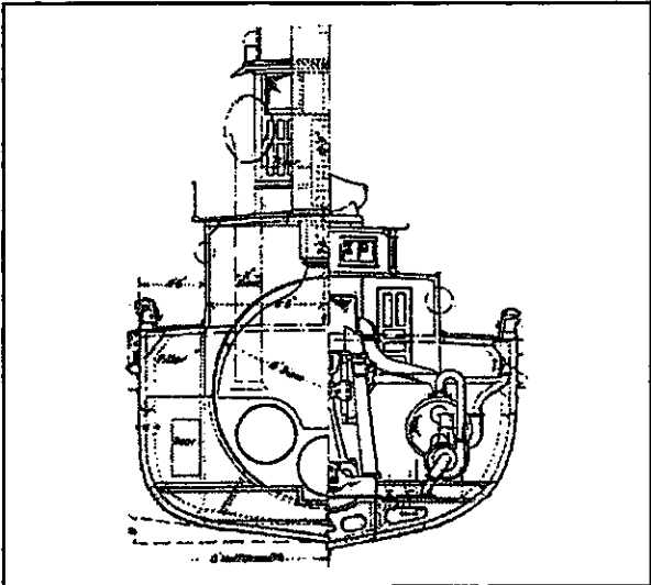
Figure 20. Midship section of the tug Newark (International Marine Engineering 1916).
