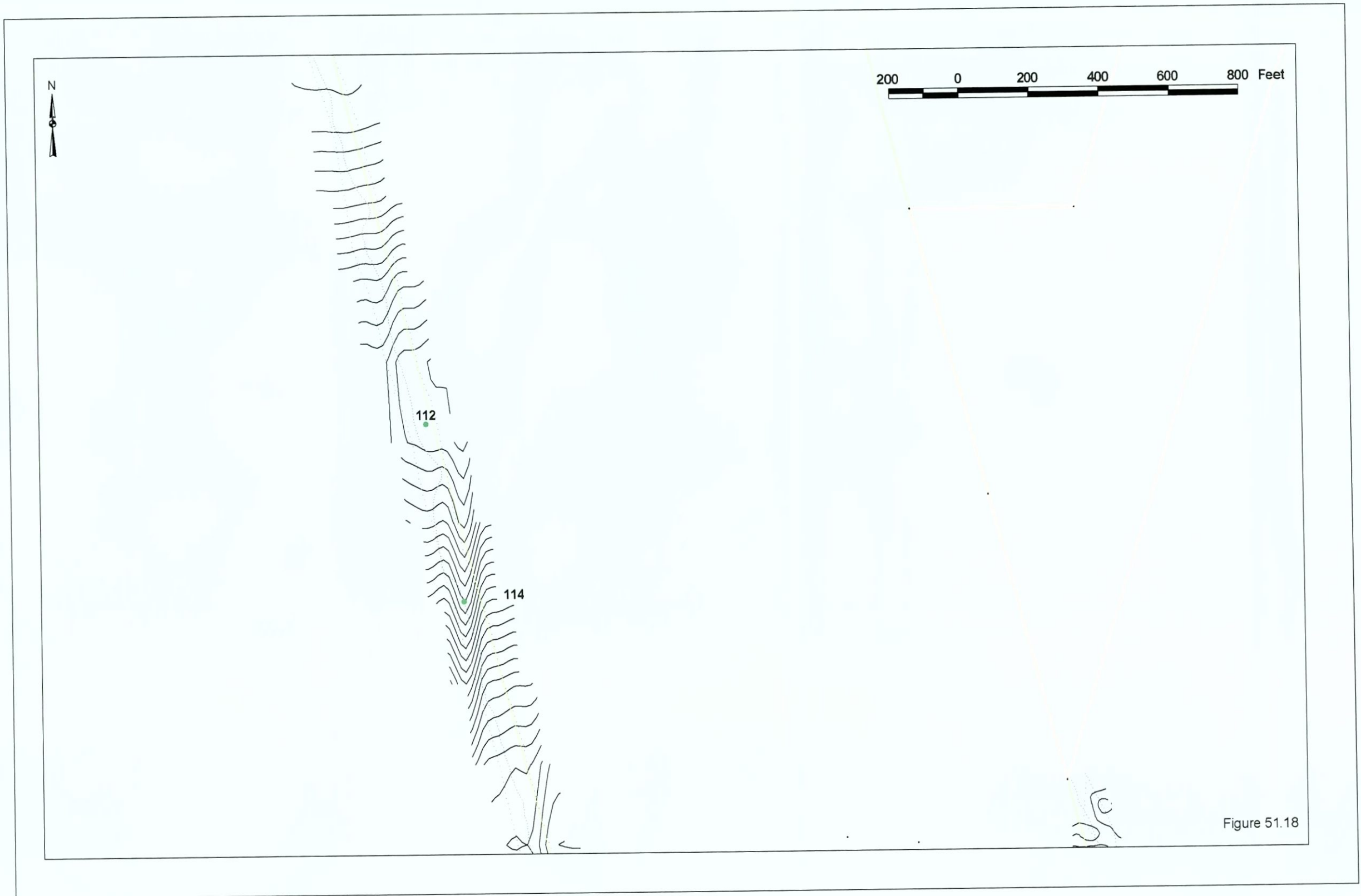
Figure 51.18. Magnetic contour map of the project area.
