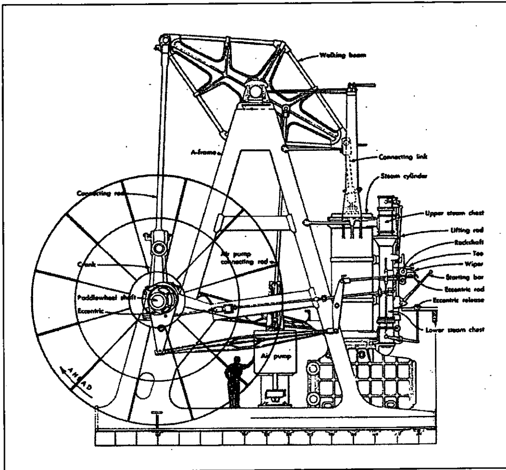
Figure 17. Labeled illustration of a walking beam engine of intermediate size (as presented in Whittier 1987:50).
