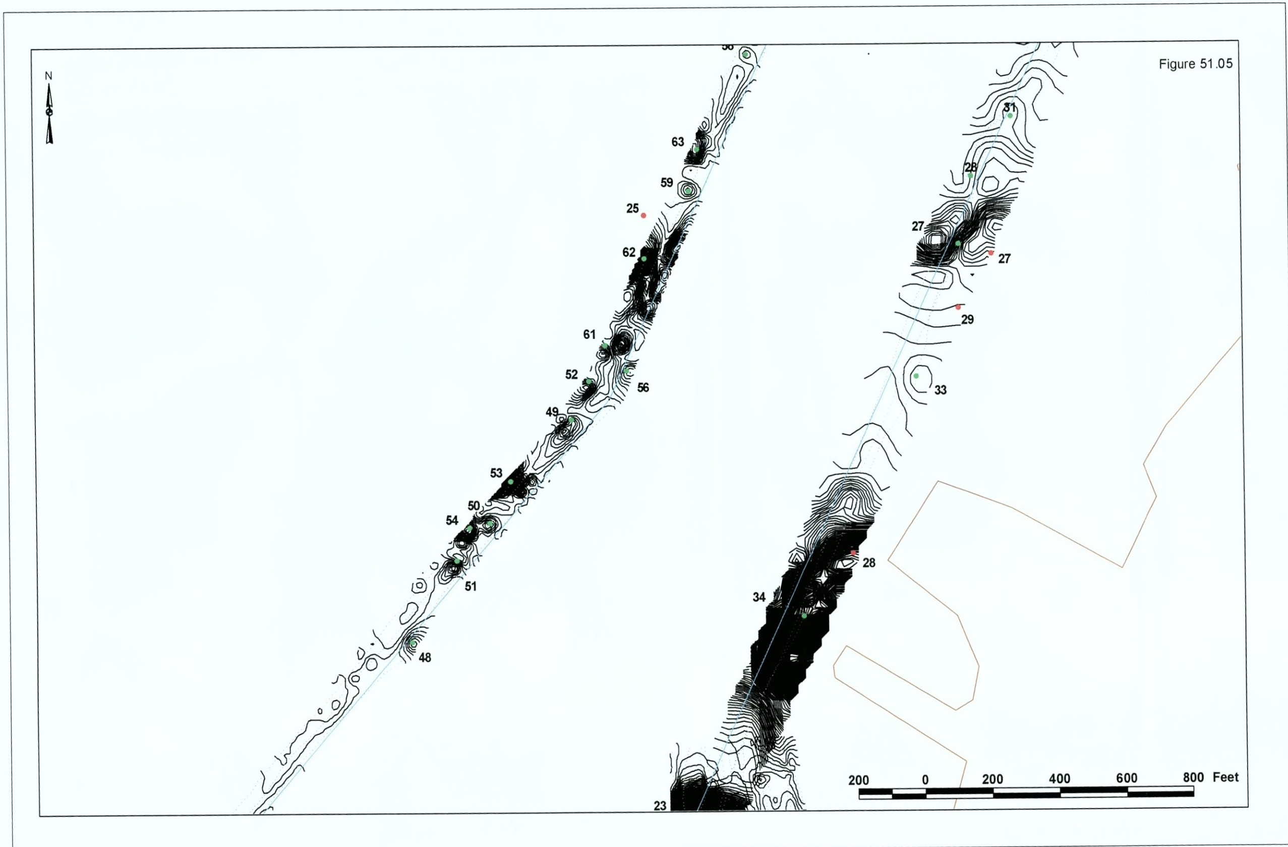
Figure 51.05. Magnetic contour map of the project area.
