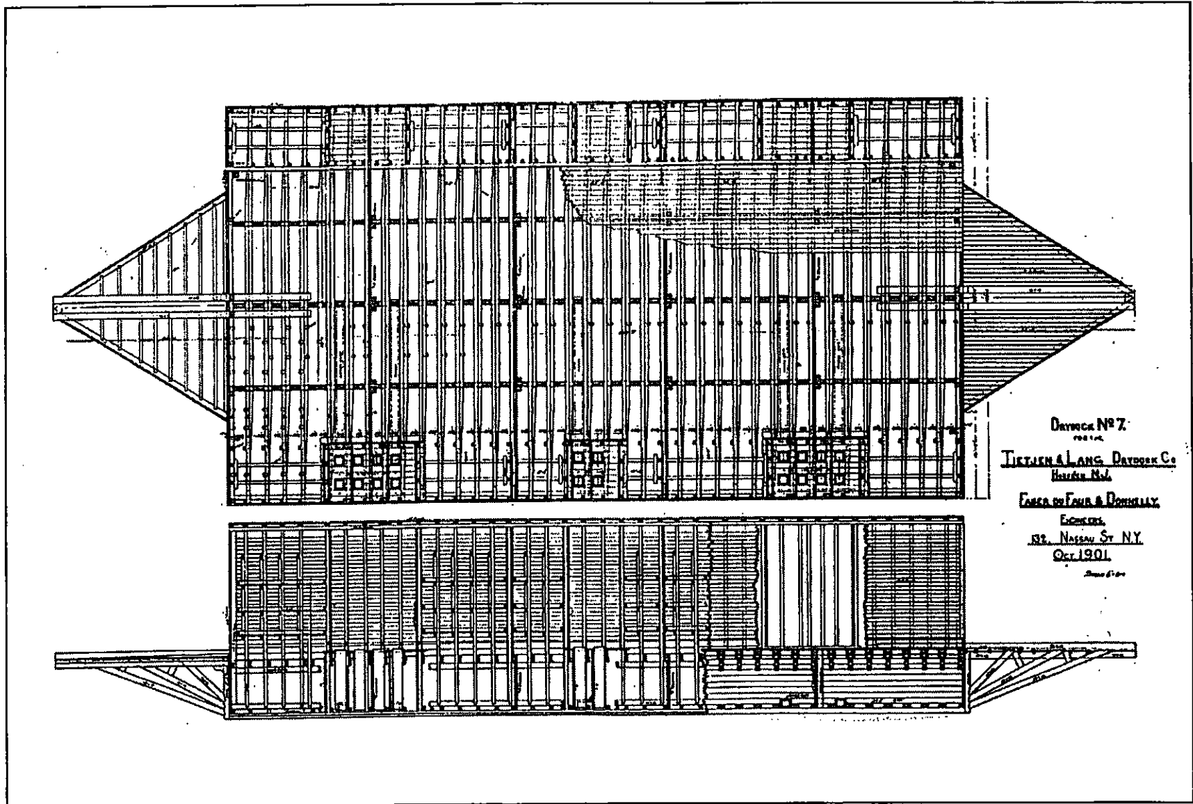
Figure 30. Plan and structural view of a box or balanced floating dry dock designed for the Tietjen and Lang Drydock Company in Hoboken, New Jersey, 1901 (as presented in Donnelly 1905).
