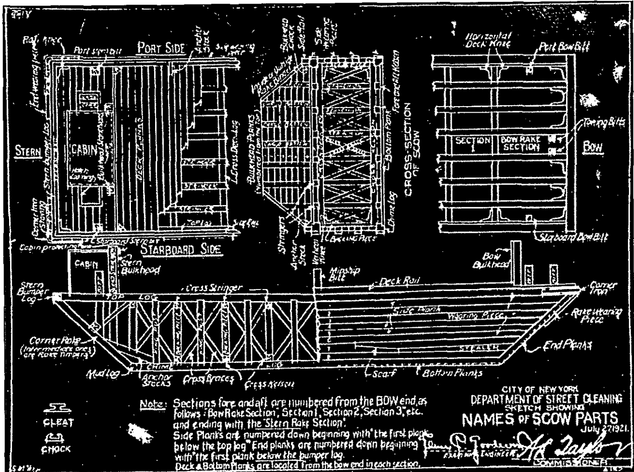
Figure 4. Plan of a 1921 street-cleaning scow (NYC Department of Street Cleaning 1921).
