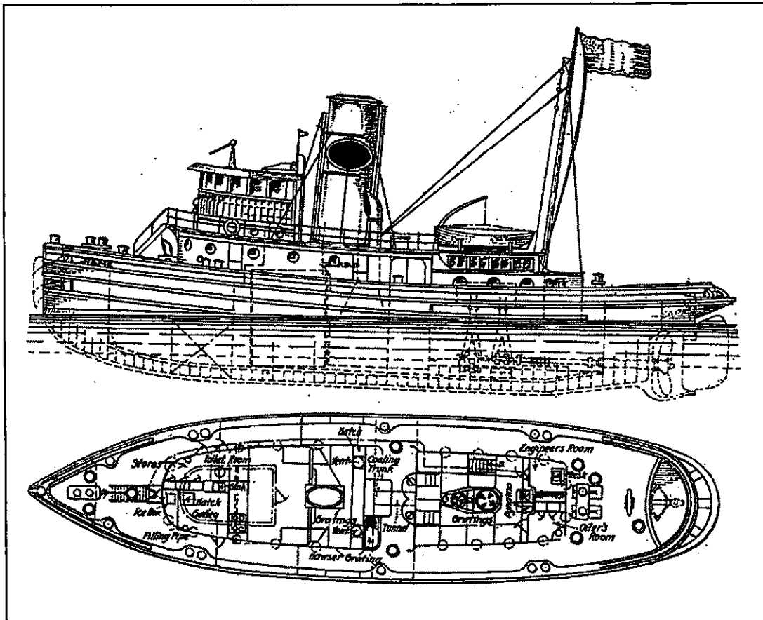
Figure 21. General arrangement of the iron-hulled Newark (International Marine Engineering 1916).
