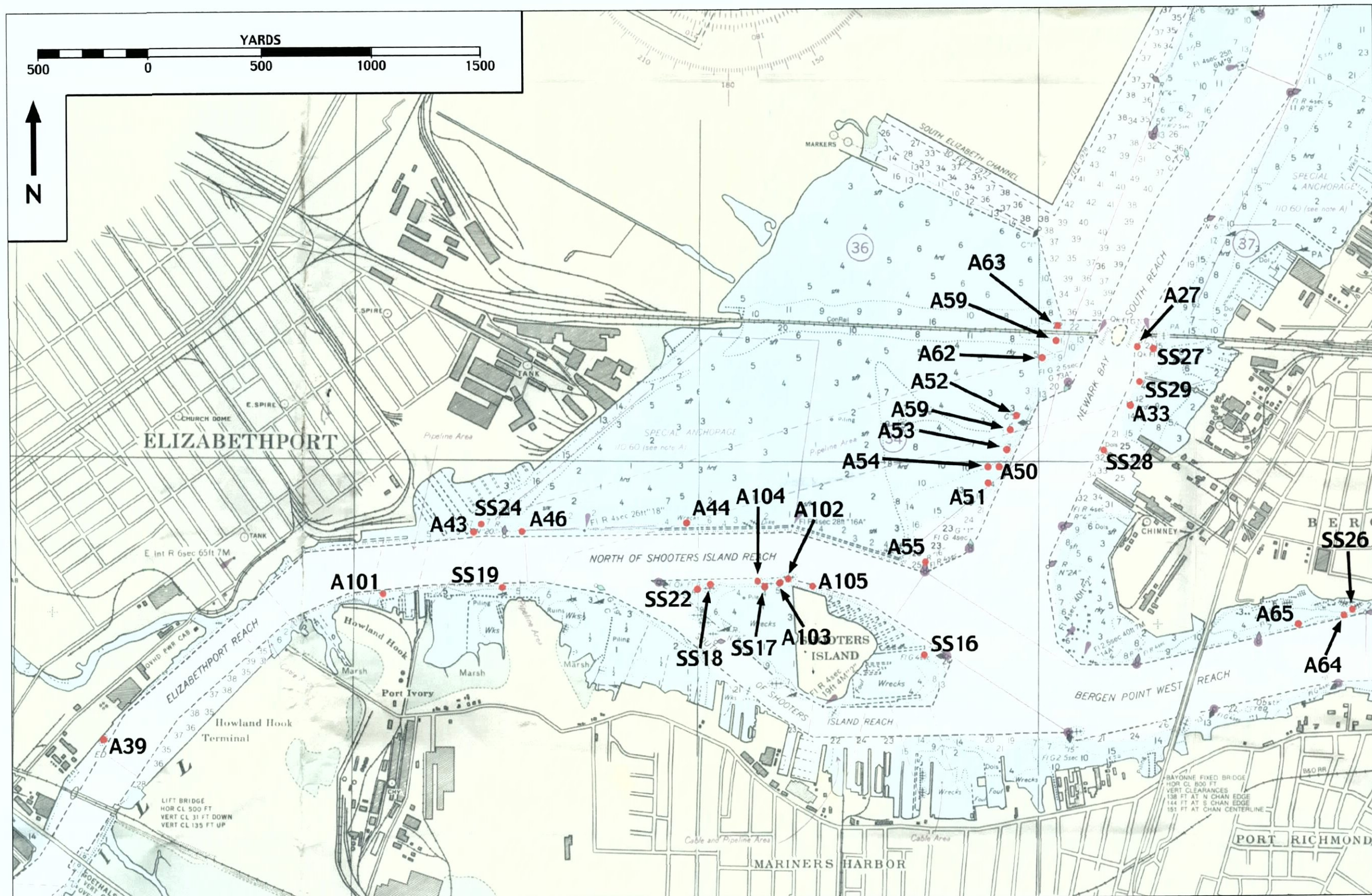
Figure 50c. Location of targets recommended for further work, map 3 of 4 (base map: NOAA Chart No. 12333, Kill Van Kull and Northern Part of Arthur Kill).
